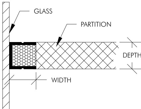
1 THREE SIDE COATED EXAMPLE N.T.S.
